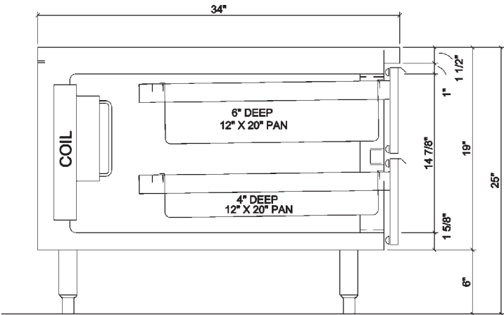
Side View VSRB SERIES
