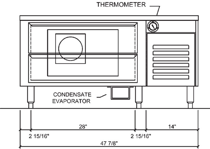
Front View VSRB48
