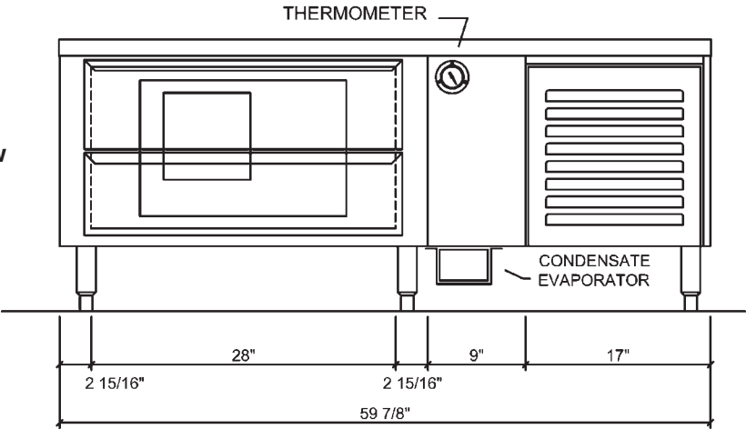
Front View VSRB60
