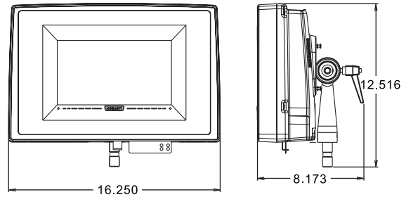
EPCP-5i Front View
