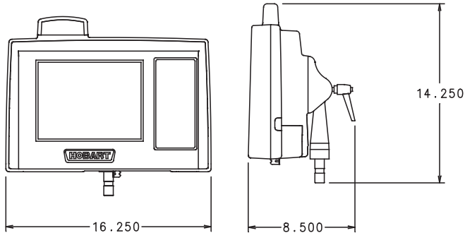
EPCP-3 & EPCP-4 Front View
