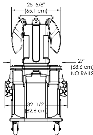
END VIEWS
